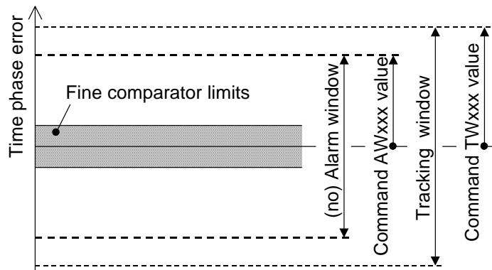
Figure 6 - Tracking Limits
