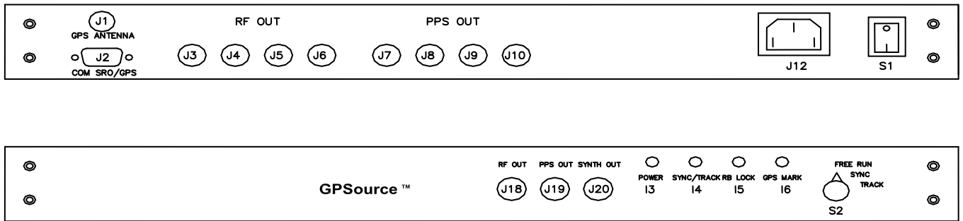
Figure 8 - GPSReference-2000 Interfaces
